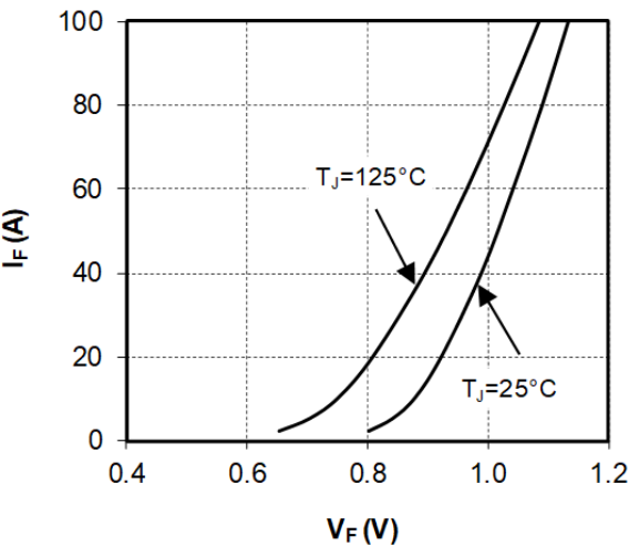
Figure 1-2. Forward Characteristics
