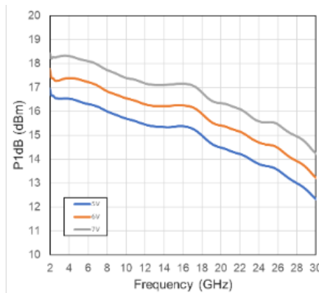
Figure 10 • P1dB vs. Drain Voltage
