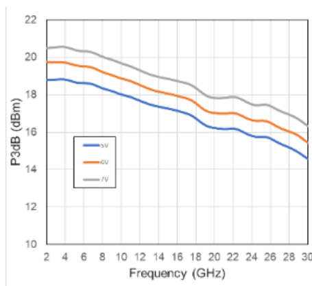
Figure 12 • P3dB vs. Drain Voltage
