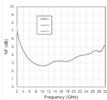
Figure 8 • Noise Figure vs. Drain Voltage
