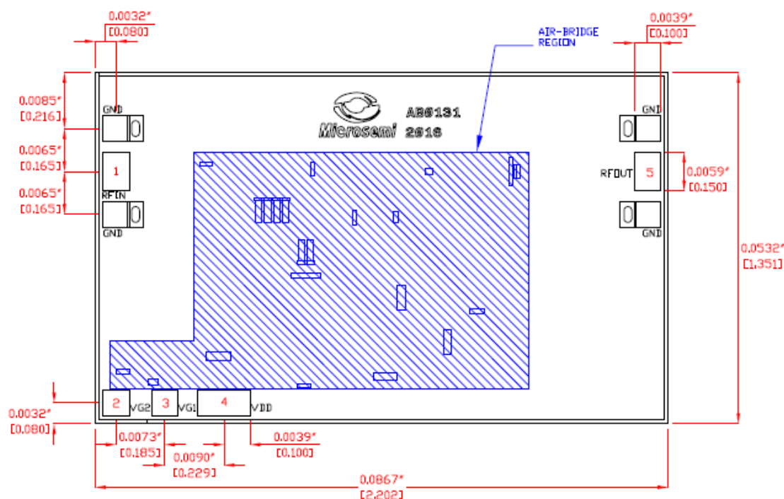
Figure 14 Chip Outline
