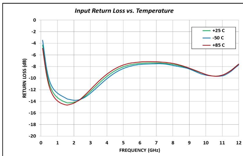
Figure 10 Input Return Loss vs. Temperature and Frequency
