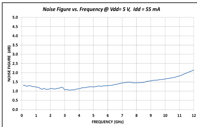
Figure 6 Noise Figure vs. Frequency
