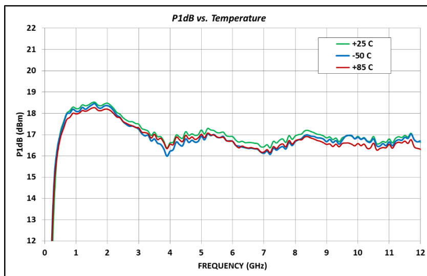
Figure 12 P1dB vs. Temperature and Frequency
