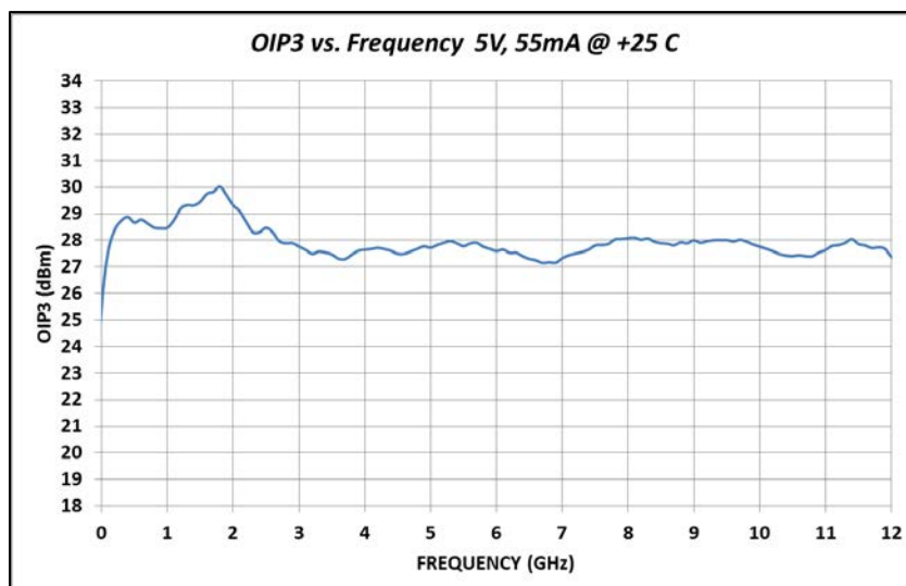
Figure 8 OIP3 vs. Frequency
