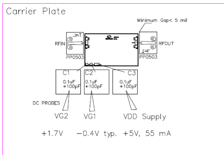
Figure 15 Assembly Diagram
