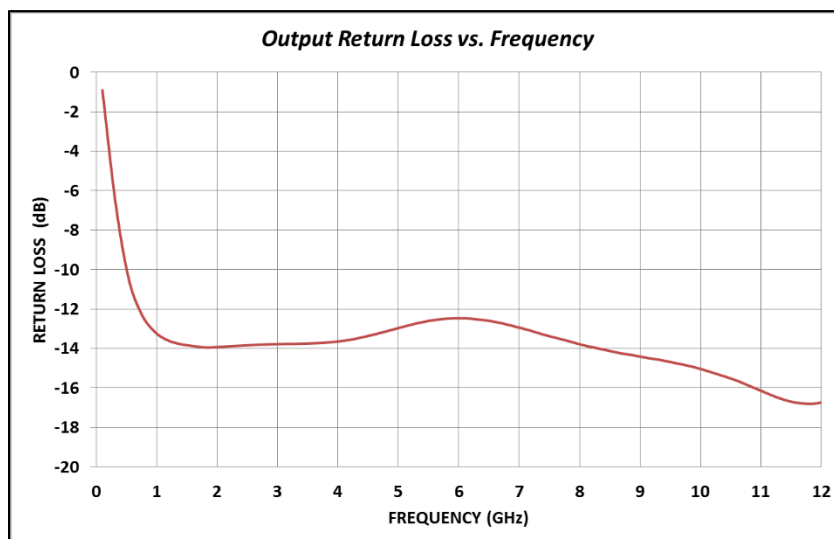
Figure 4 Output Return Loss vs. Frequency
