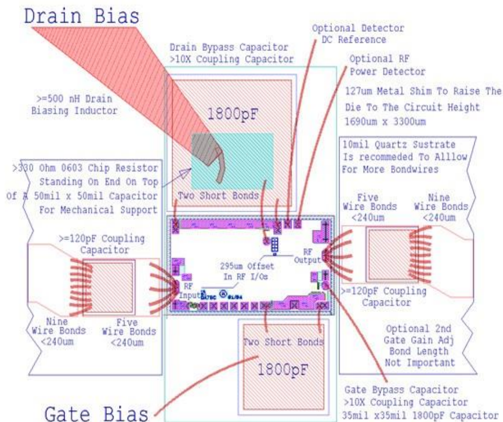
Figure 3. 40MHz-65GHz bonding diagram
