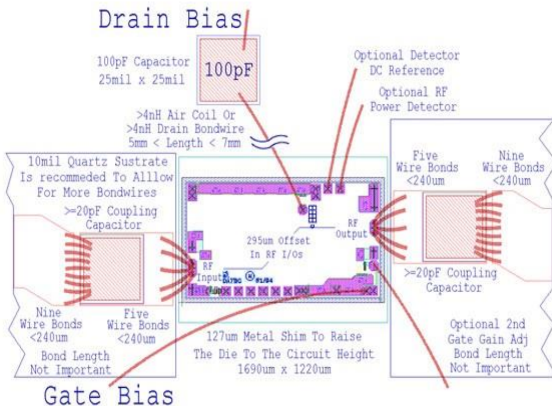
Figure 2.2 -65GHz bonding diagram
