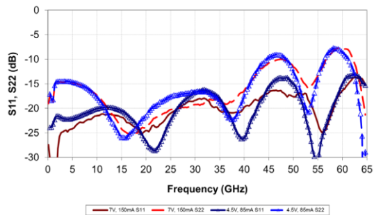
S11, S22
