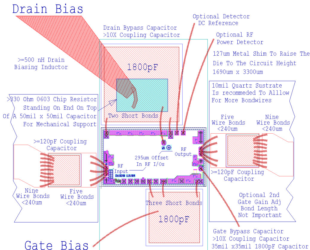
Figure 3. 40MHz-65GHz bonding diagram
