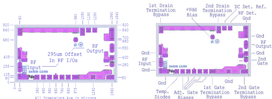
Figure 1. Die size, pad locations, and pad descriptions
