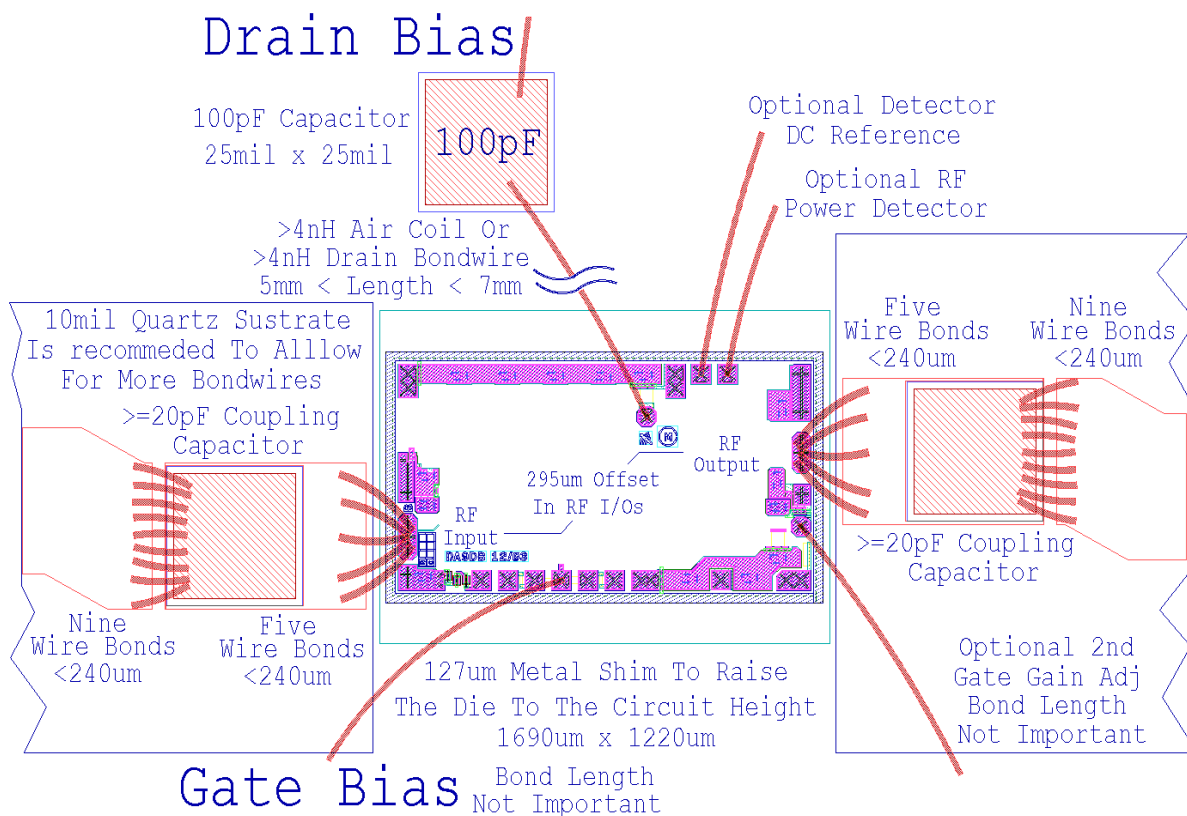
Figure 2.2 -65GHz bonding diagram
