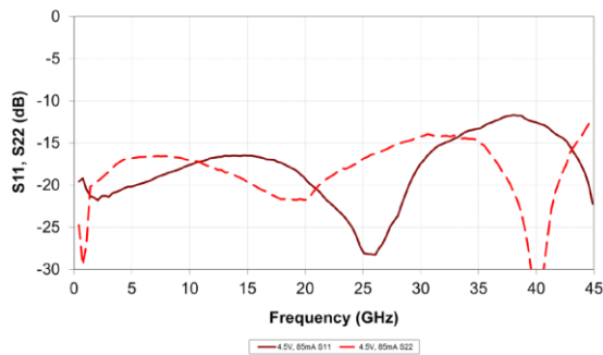
S11, S22
