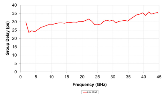
Group Delay
