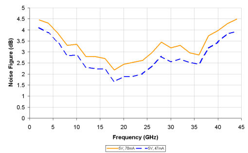
Noise Figure
