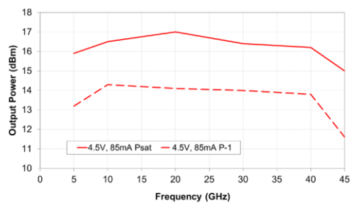
Output Power
