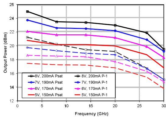
Output Power
