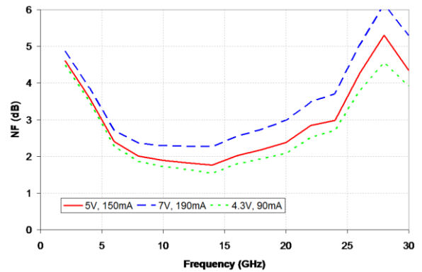
Noise Figure
