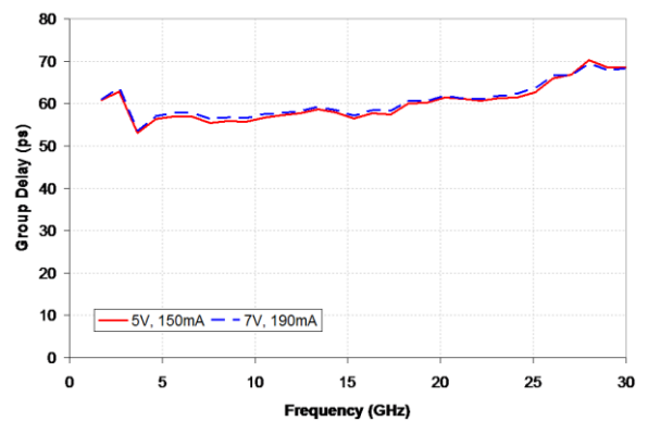
Group Delay
