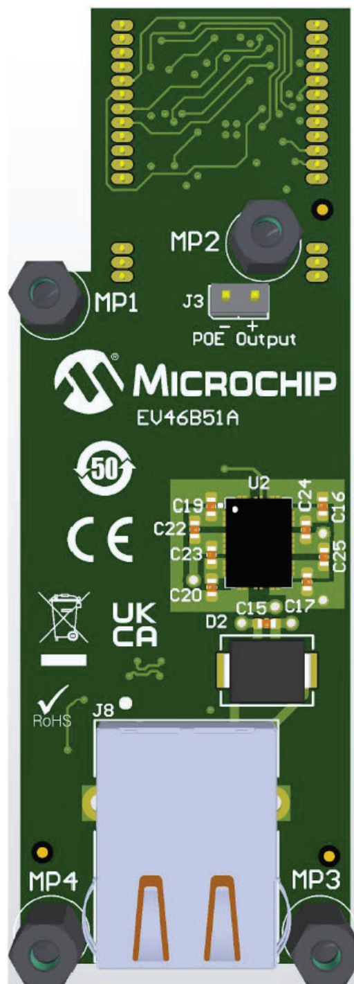
Figure 3. EV46B51A Evaluation Board—Bottom View
