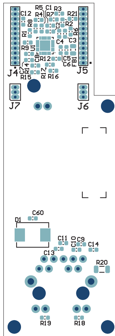
Figure 5-6. Bottom Board—Bottom Silk
