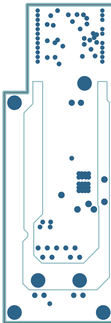
Figure 5-8. Bottom Board—Middle Layer 1 Copper
