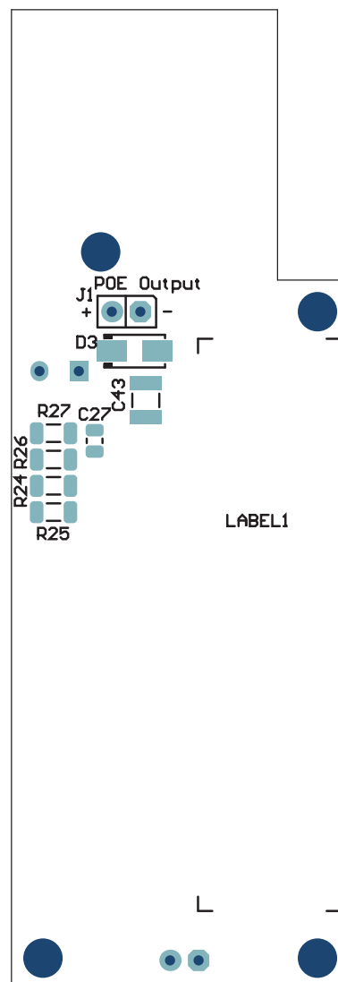
Figure 5-2. Top Board—Bottom Silk
