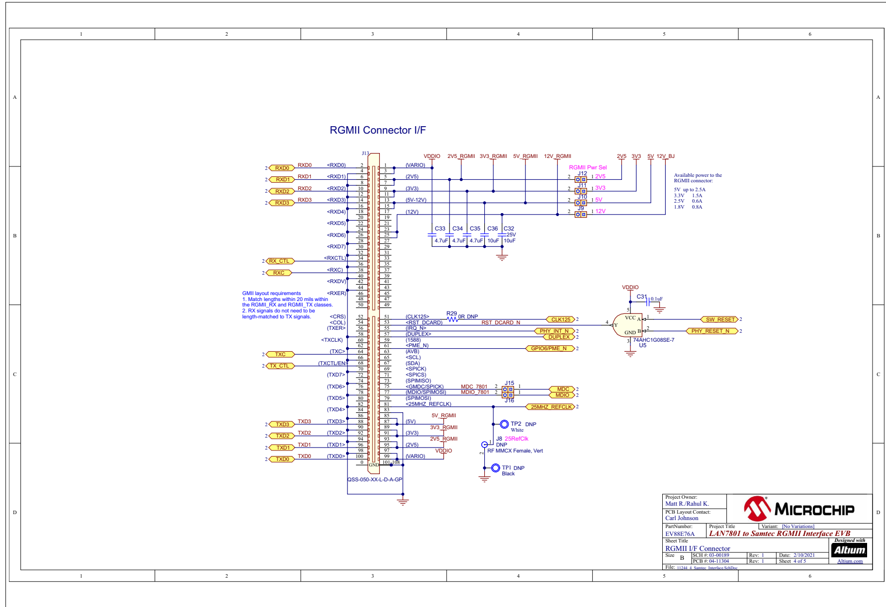
FIGURE B-4: RGMII/IF CONNECTOR
