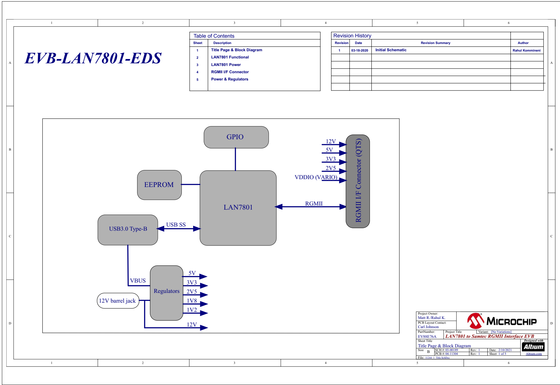
FIGURE B-1: EVB-LAN7801-EDS BLOCK DIAGRAM
