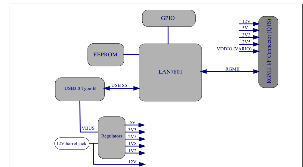
FIGURE 1-1: EVB-LAN7801-EDS BLOCK DIAGRAM
