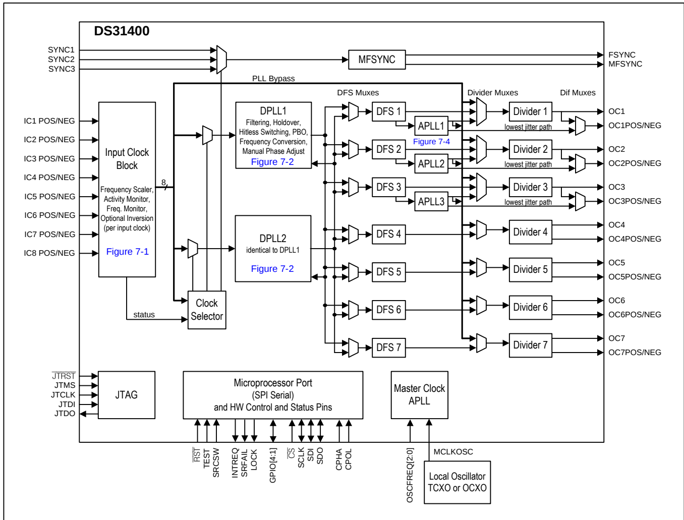
Figure 3-1. DS31400 Block Diagram
