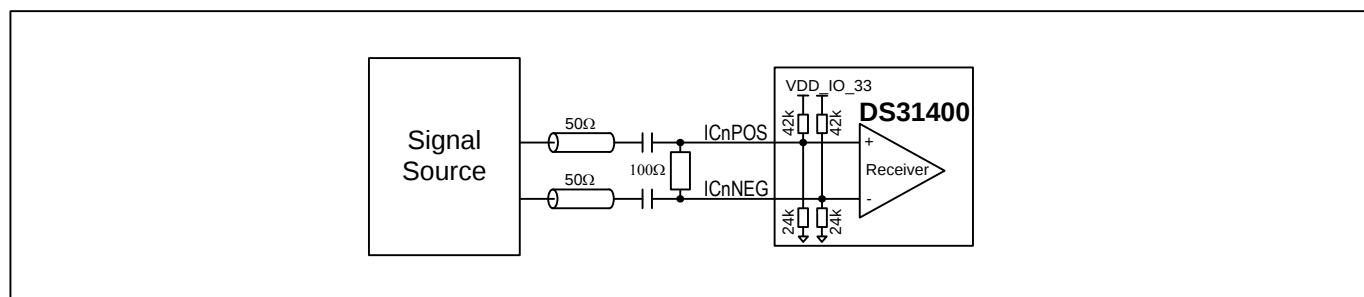
Figure 10-1. Recommended External Components for Interfacing to Differential Inputs
