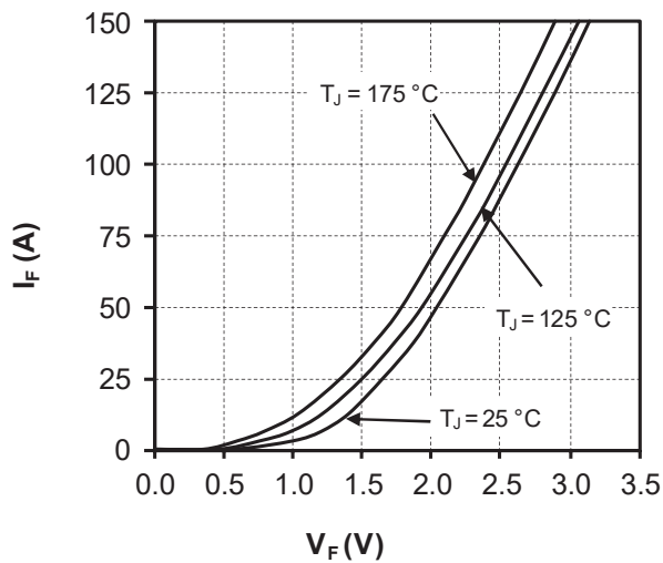
Figure 1-12. Forward Characteristics
