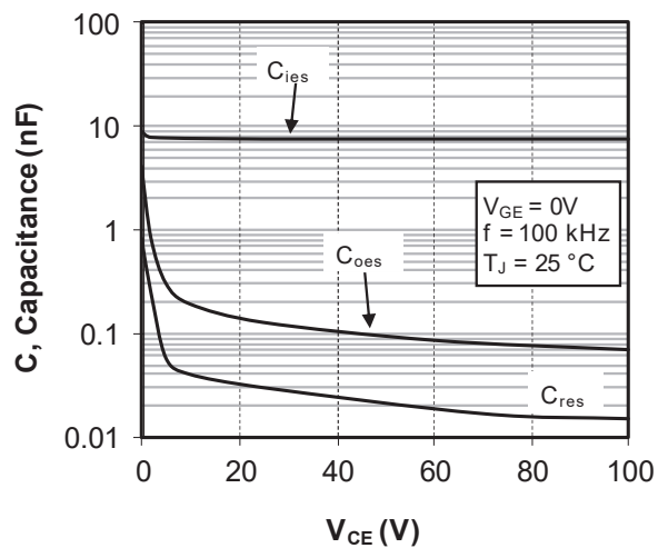
Figure 1-9. Capacity Characteristics
