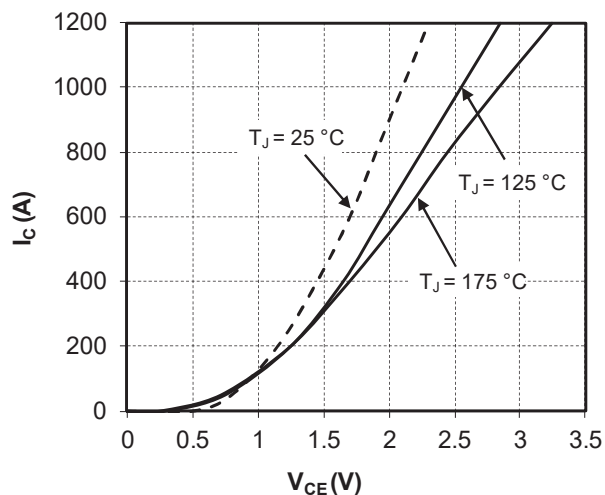
Figure 1-2. Output Characteristics, V_{GE} = 15\text{V}
