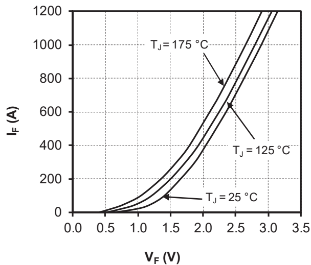
Figure 1-12. Forward Characteristics
