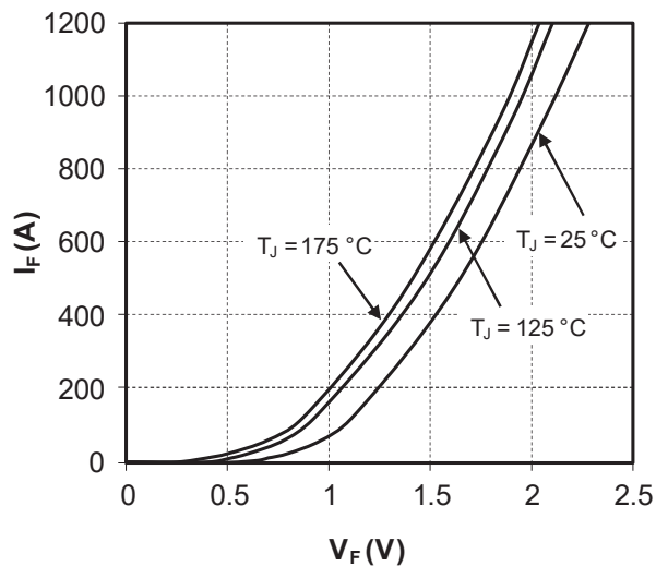
Figure 1-12. Forward Characteristics
