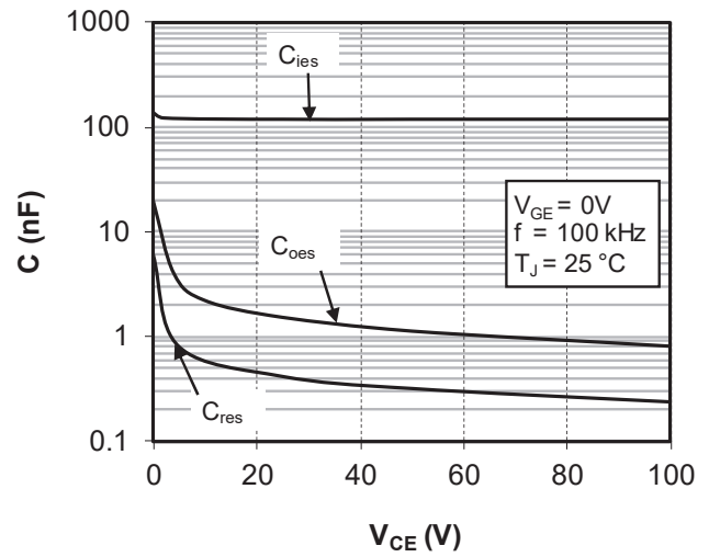
Figure 1-9. Capacity Characteristics
