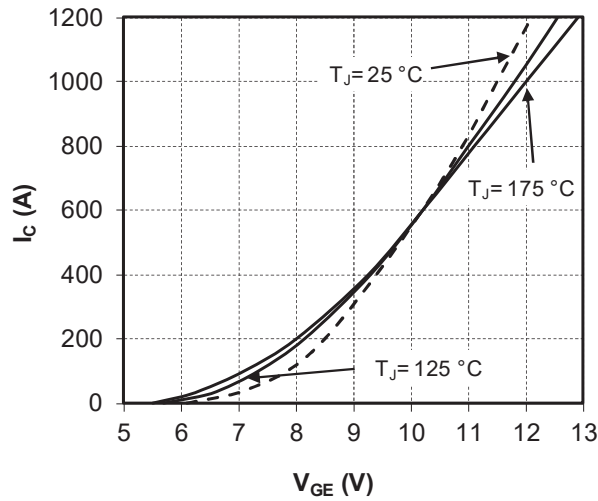
Figure 1-8. Transfer Characteristics
