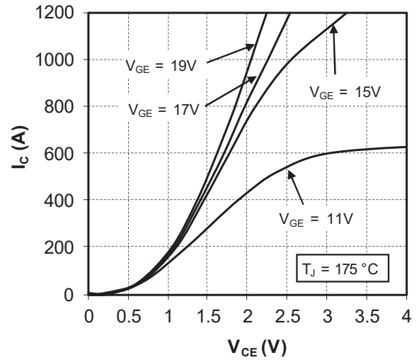
Figure 1-3. Output Characteristics, T_J = 175\text{ °C}
