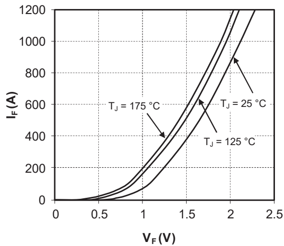
Figure 1-12. Forward Characteristics
