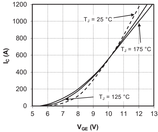
Figure 1-8. Transfer Characteristics
