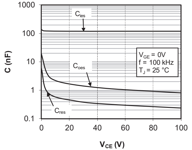
Figure 1-9. Capacity Characteristics
