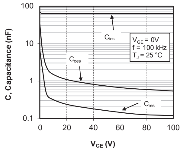
Figure 1-9. Capacity Characteristics
