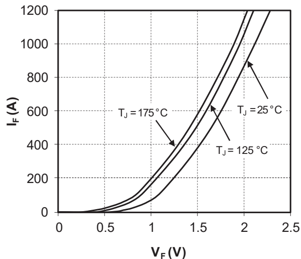
Figure 1-12. Forward Characteristics
