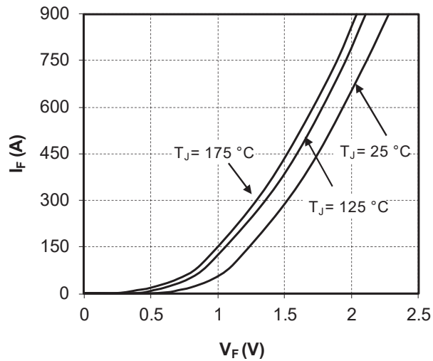
Figure 1-12. Forward Characteristics
