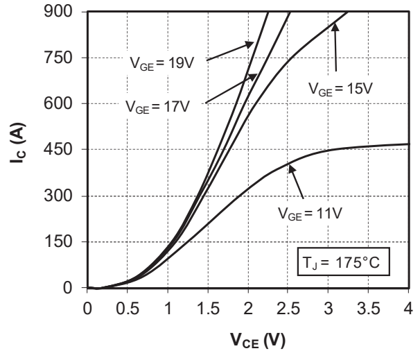
Figure 1-3. Output Characteristics, T_J = 175^\circ C
