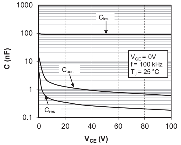
Figure 1-9. Capacity Characteristics
