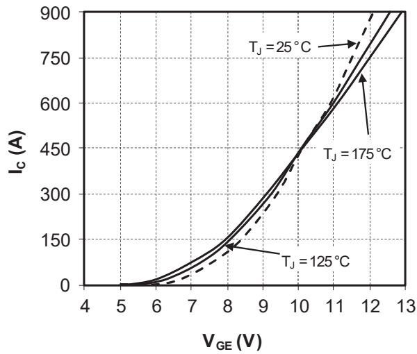
Figure 1-8. Transfer Characteristics
