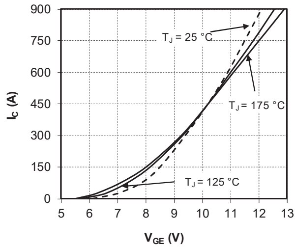
Figure 1-8. Transfer Characteristics
