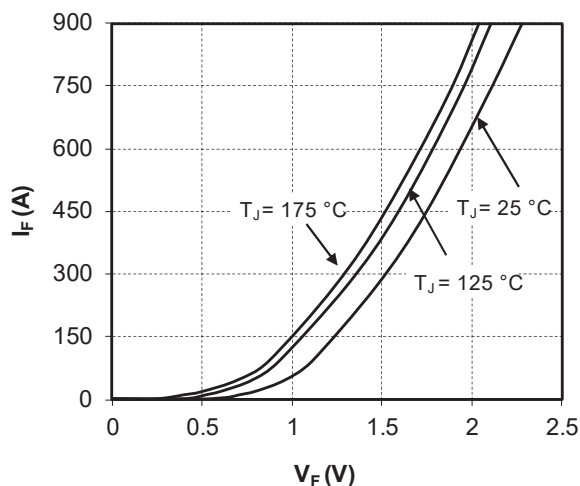
Figure 1-12. Forward Characteristics
