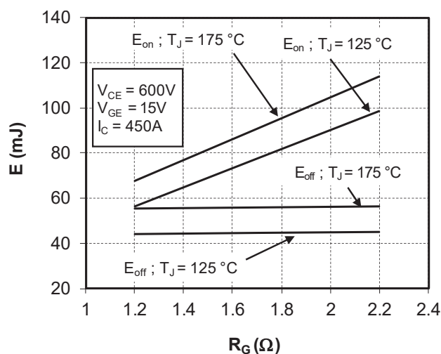
Figure 1-4. Switching Losses vs. Gate Resistance
