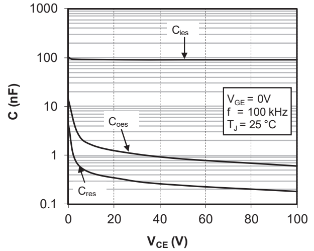
Figure 1-9. Capacity Characteristics
