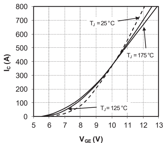
Figure 1-8. Transfer Characteristics
