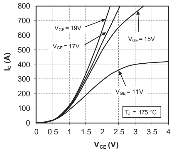
Figure 1-3. Output Characteristics, T_J = 175^{\circ}\text{C}
