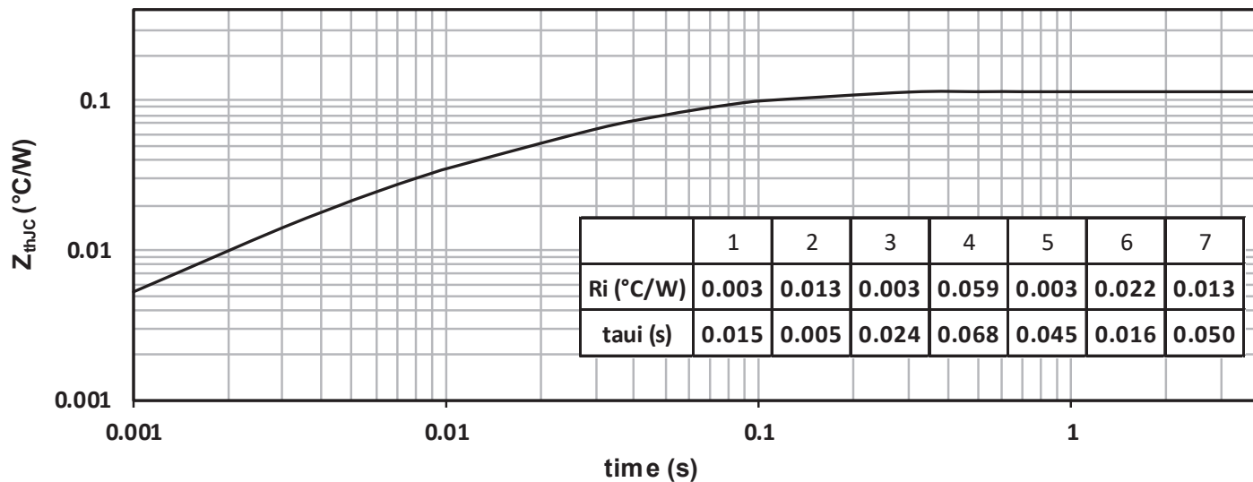
Figure 1-1. Maximum Thermal Impedance
