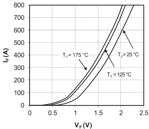
Figure 1-12. Forward Characteristics
