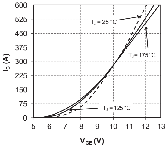
Figure 1-8. Transfer Characteristics
