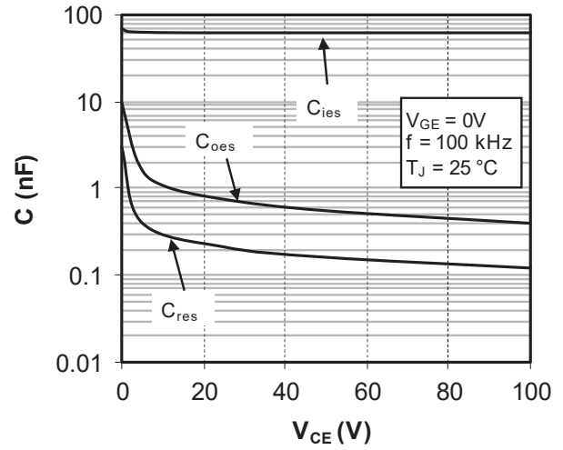
Figure 1-9. Capacity Characteristics
