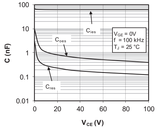
Figure 1-9. Capacity Characteristics
