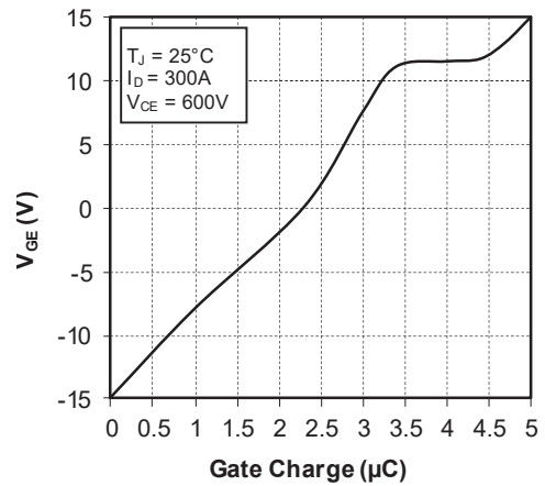
Figure 1-7. Gate Charge Characteristics
