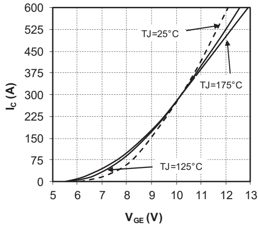
Figure 1-8. Transfer Characteristics
