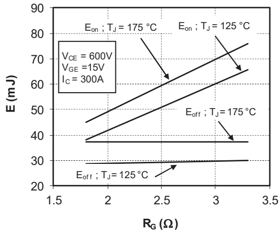
Figure 1-4. Switching Losses vs. Gate Resistance
