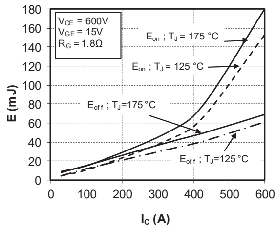
Figure 1-5. Switching Losses vs. Collector Current
