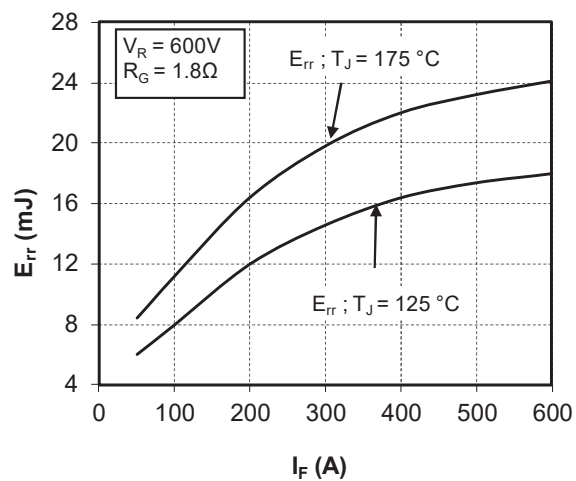
Figure 1-14. Switching Losses vs. Forward Current
