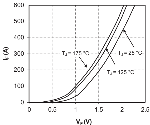
Figure 1-12. Forward Characteristics
