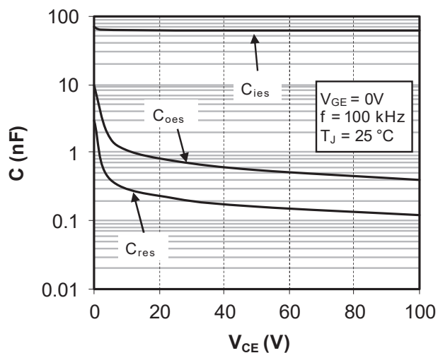
Figure 1-9. Capacity Characteristics
