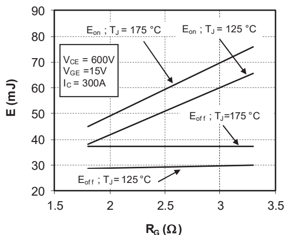
Figure 1-4. Switching Losses vs. Gate Resistance
