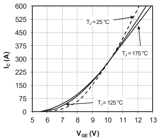
Figure 1-8. Transfer Characteristics
