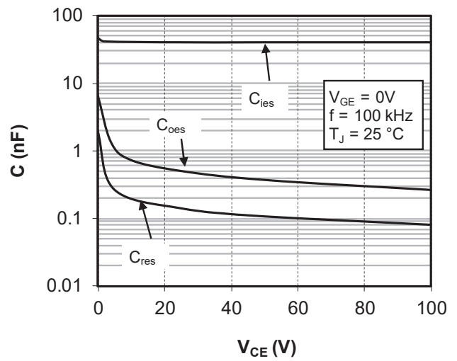
Figure 1-9. Capacity Characteristics
