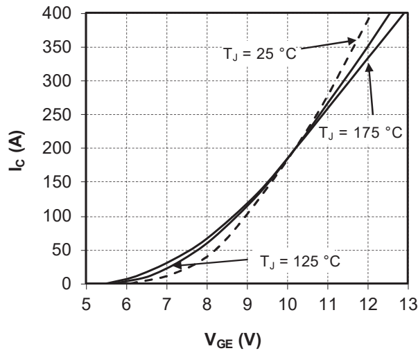
Figure 1-8. Transfer Characteristics
