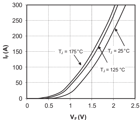
Figure 1-12. Forward Characteristics
