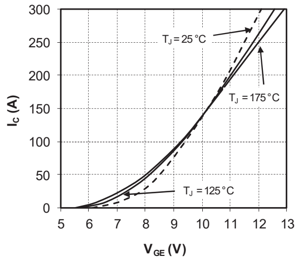
Figure 1-8. Transfer Characteristics
