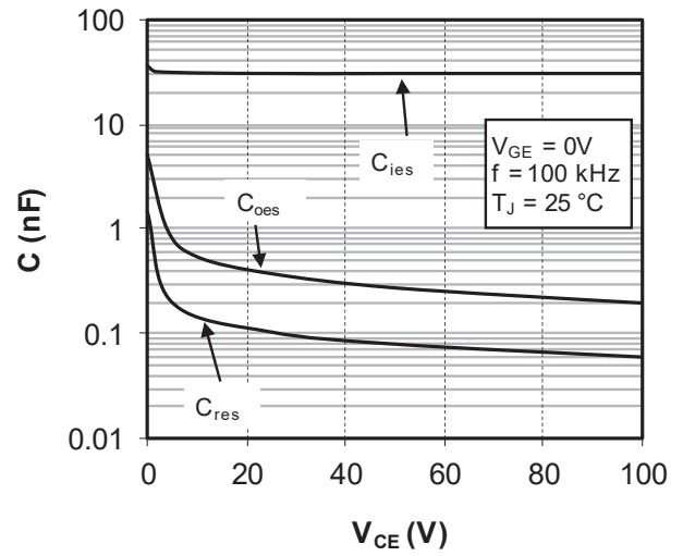
Figure 1-9. Capacity Characteristics
