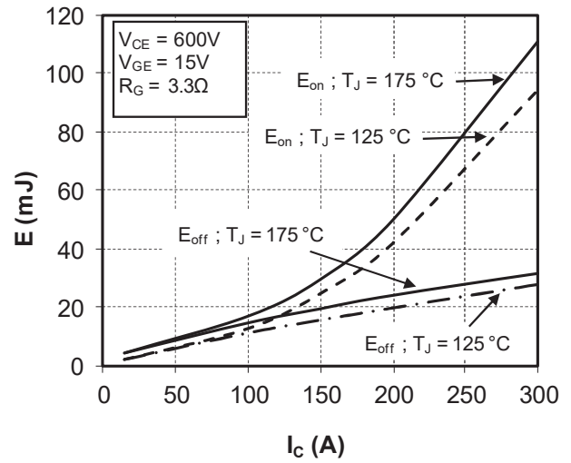
Figure 1-5. Switching Losses vs. Collector Current
