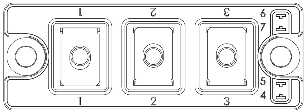
Figure 2. Pinout Location
