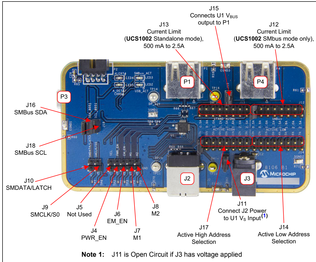
FIGURE 2-3: Evaluation Board Top View - Jumpers.
