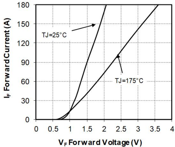
Figure 1-16. Forward Characteristics
