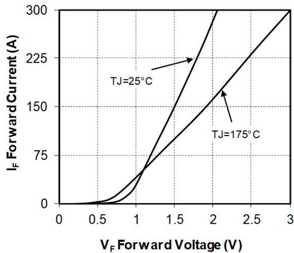
Figure 1-17. Forward Characteristics
