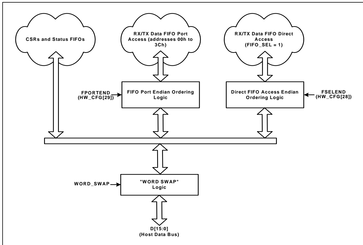
FIGURE 3-8: LAN9210 HOST DATA PATH DIAGRAM
