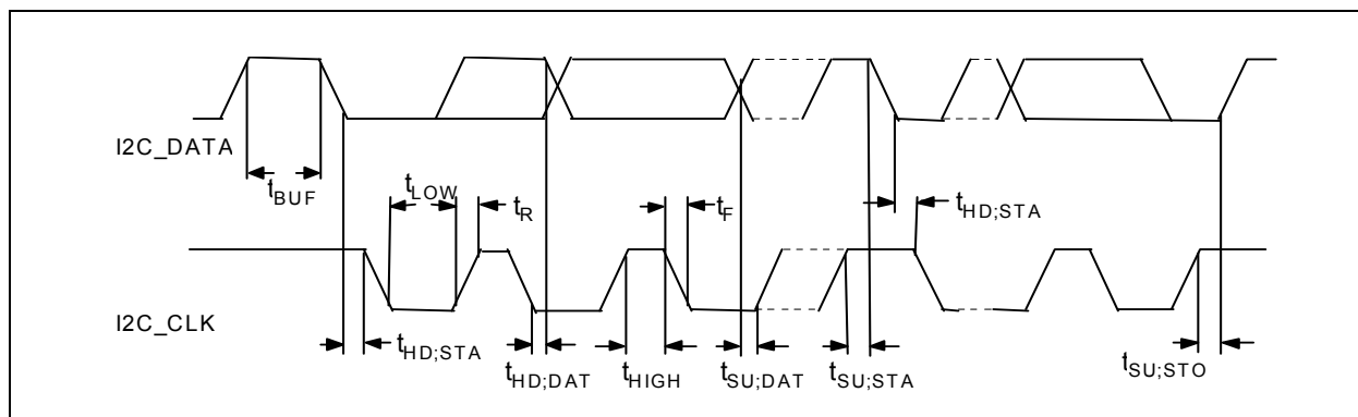
FIGURE 43-9: I 2 C/SMBUS TIMING
