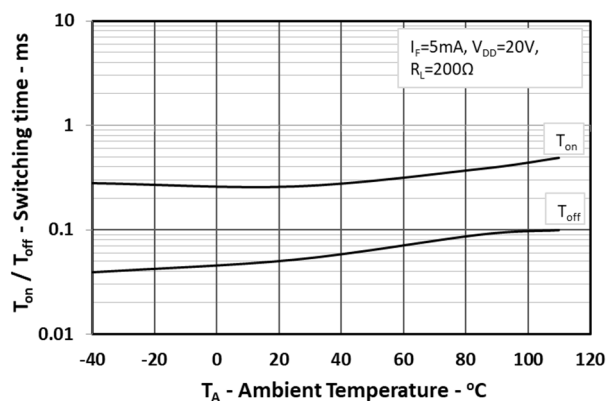
Fig. 7 Switching time vs. Ambient Temperature
