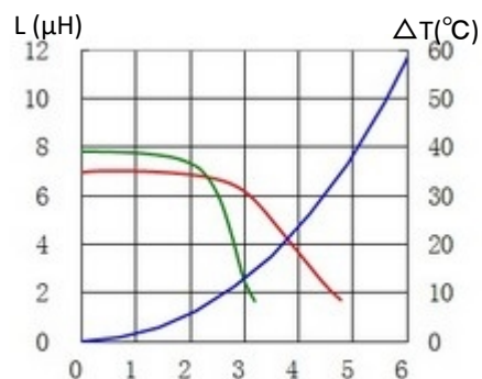
7. CDRH70D45BT150NP-6R8NC
