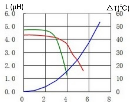
6. CDRH70D45BT150NP-4R7NC
