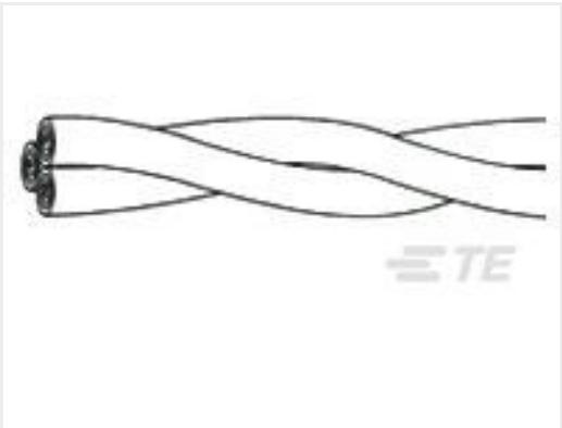
TE Part #3830593001 44A0131-22-0/2/9
