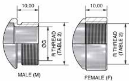
METRIC THREAD (TM)
