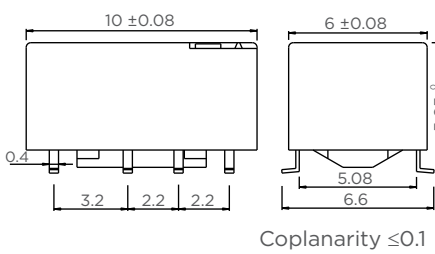
SMT Short Gull wings version
