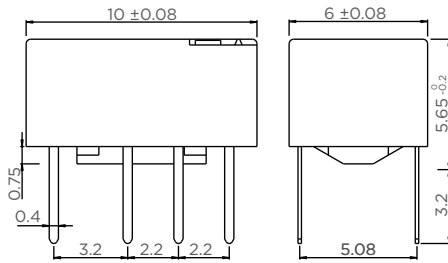
THT Standard version
