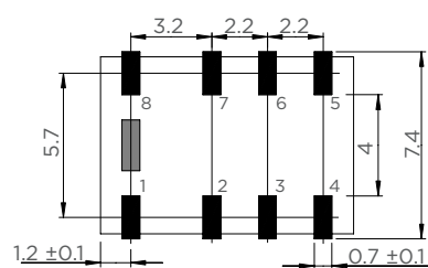
SMT Short Gull wings version
