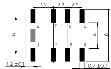
SMT Gull wings version
