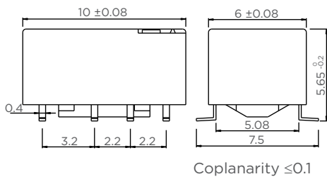
SMT Gull wings version
