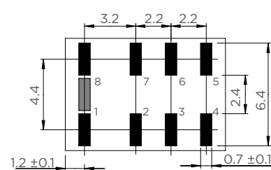
SMT J-legs version
