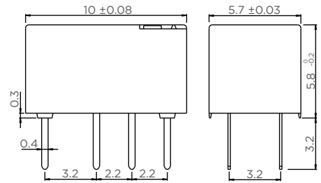
THT Narrow version
