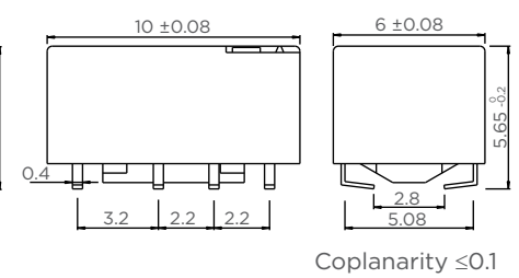
SMT J-legs version
