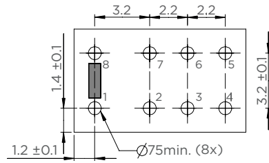
THT Narrow version
