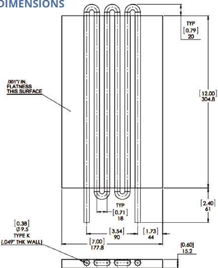
MECHANICAL DIMENSIONS
