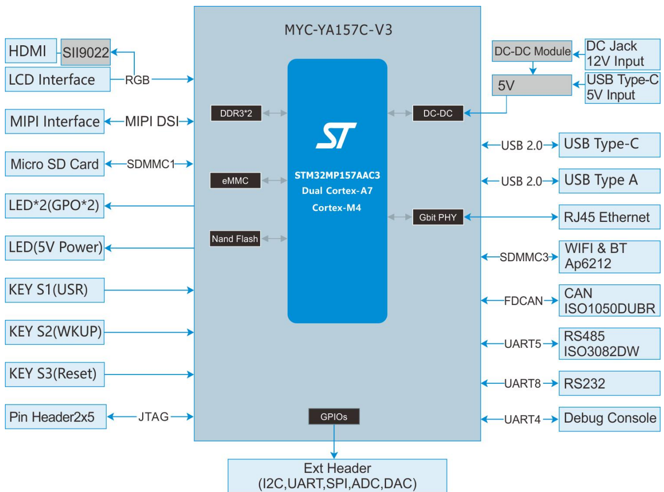
MYD-YA157C-V3 Development Board
