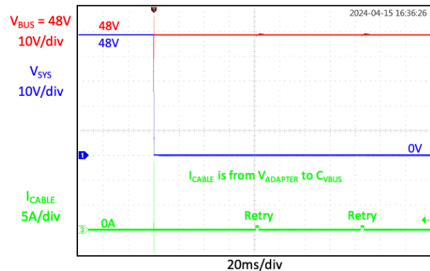
SCP & Auto-Retry Response in ISINK Mode ( V_{BUS} = 48V , V_{SYS} = sudden short circuit)
