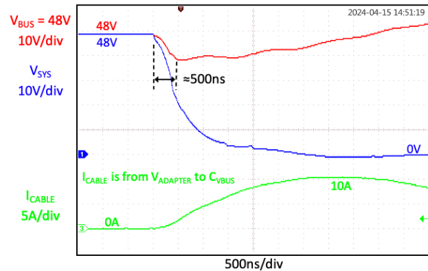
OCP/SCP Response in ISINK Mode ( V_{BUS} = 48V , V_{SYS} = sudden short circuit)
