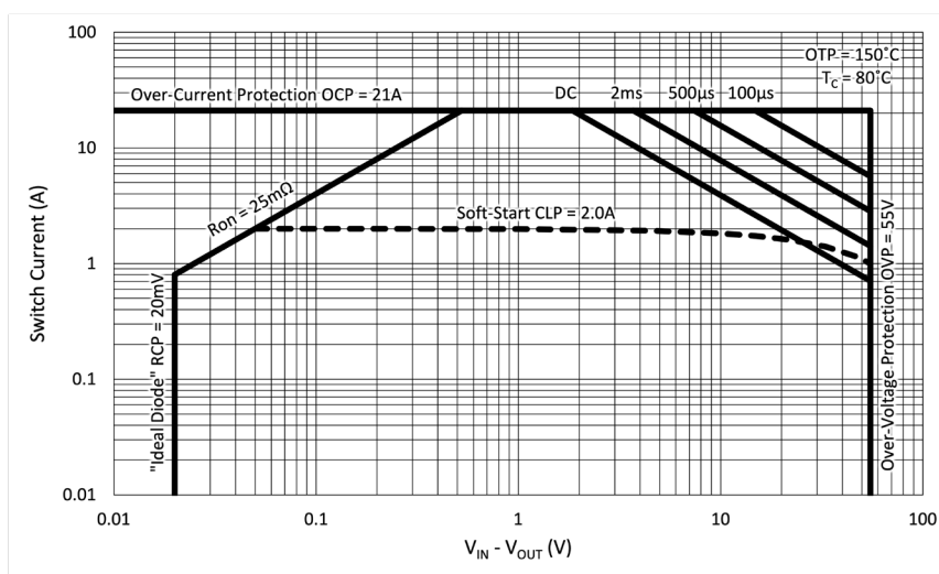
Figure 7. Safe Operating Area (SOA) for T_c = 80^\circ\text{C}
