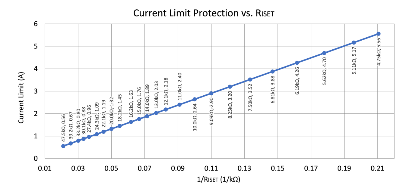
Figure 4. I SOURCE Mode Current Limit Protection vs. R ISET Resistance
