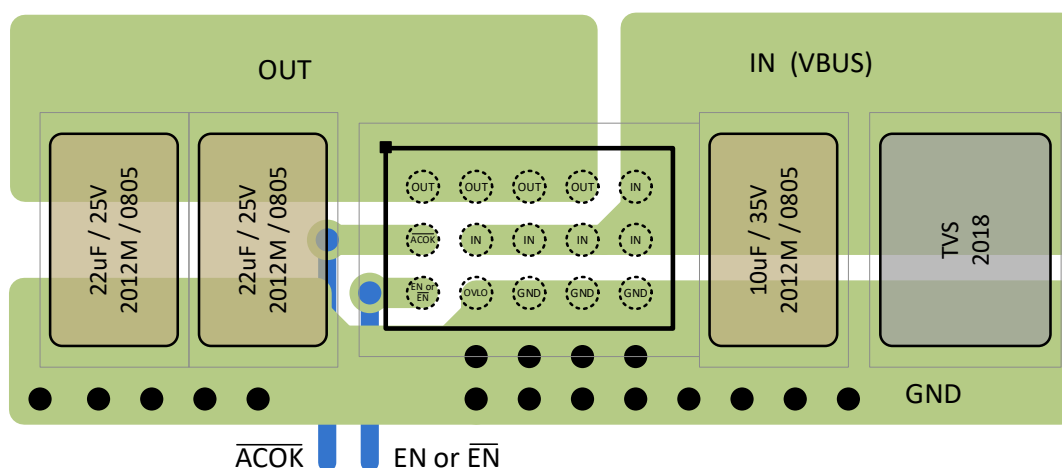
Figure 9. Recommended PCB Layout
