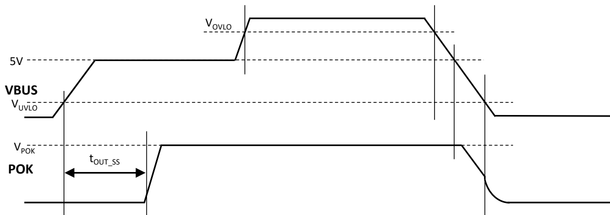
Figure 3. POK Always ON Timing ( \overline{\text{EN1}} = \text{X} , \text{EN2} = \text{X} , \text{SHDN} = \text{LOW} )
