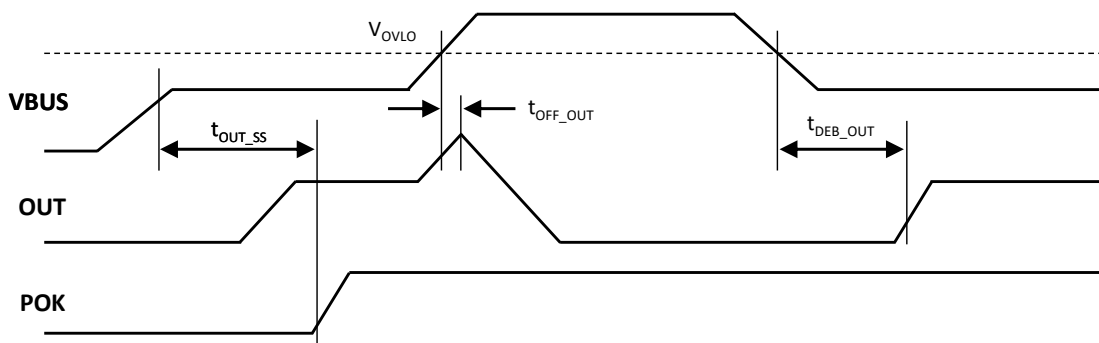
Figure 2. VBUS to OUT Timing OVLO Operation ( \overline{\text{EN1}} = \text{LOW} )
