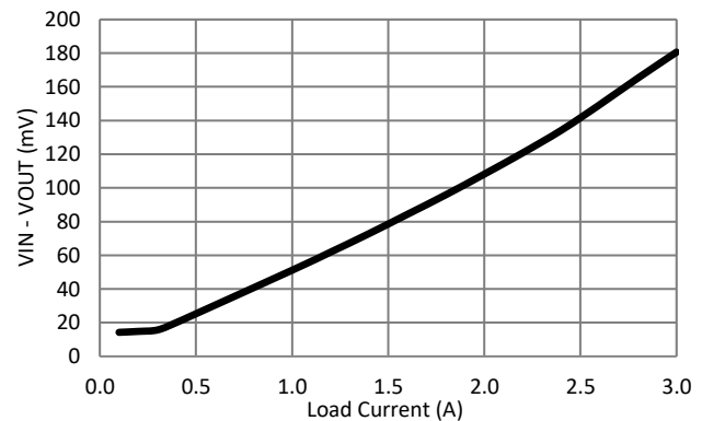
"Ideal diode" Vdroop vs. Load Current
