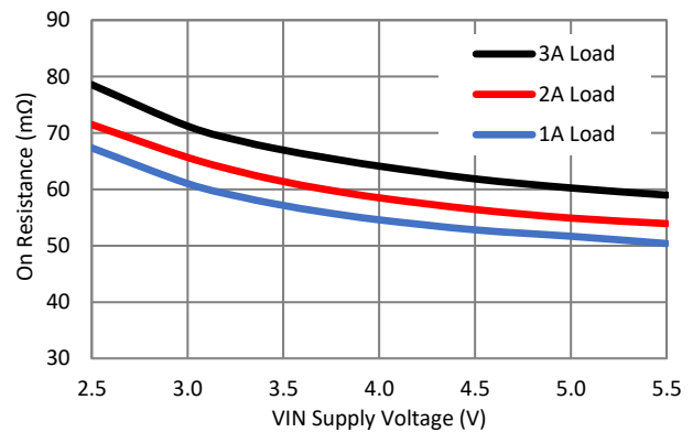
Switch On-Resistance vs. VIN
