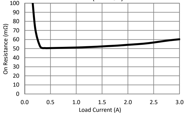
On-Resistance vs. Load Current (VIN = 5V)
