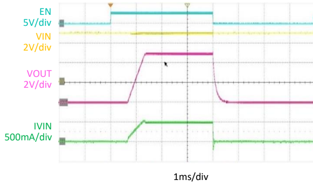
Enable Turn-on, Turn-off Response ( R_{load} = 10\Omega )
