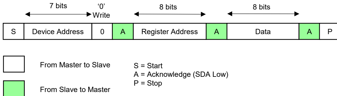
Figure 4. I 2 C Write Cycle
