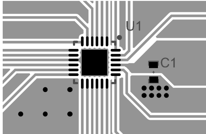
Figure 8. Recommended layout for WQFN44-24
