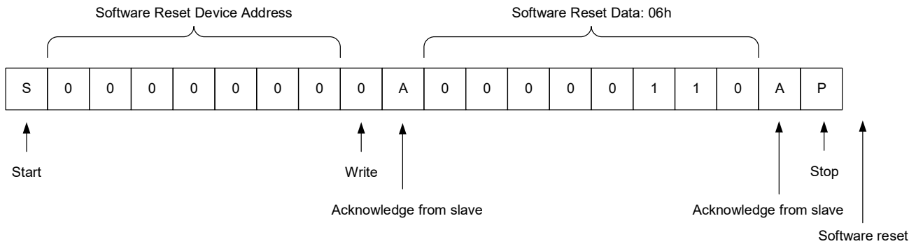
Figure 6. I 2 C Software Reset
