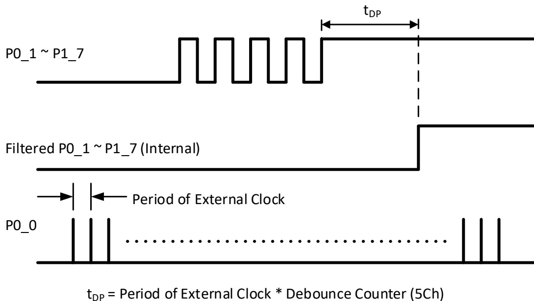
Figure 7. Debounce Timing
