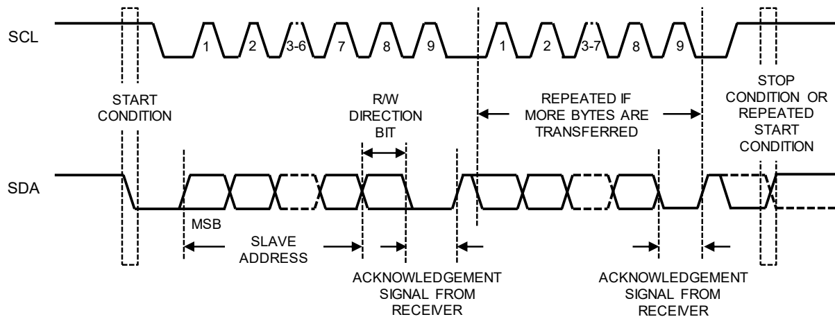
Figure 3. Data Transfer on I 2 C Serial Bus
