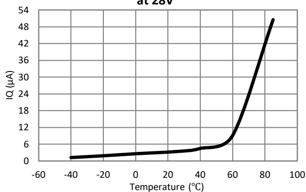
Quiescent Supply Current vs Temperature at 28V
