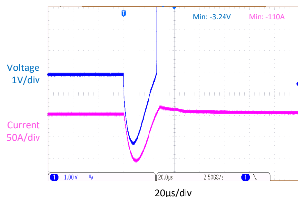
8/20 \mu s Surge Response at -110A
