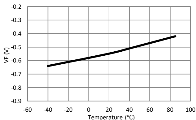
Forward Voltage (-1mA) vs Temperature
