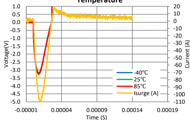
8/20 \mu s Surge Response at -110A Across Temperature
