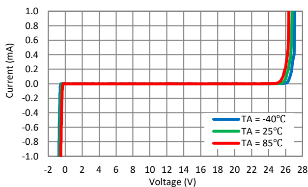
I/V Curve Across Temperature
