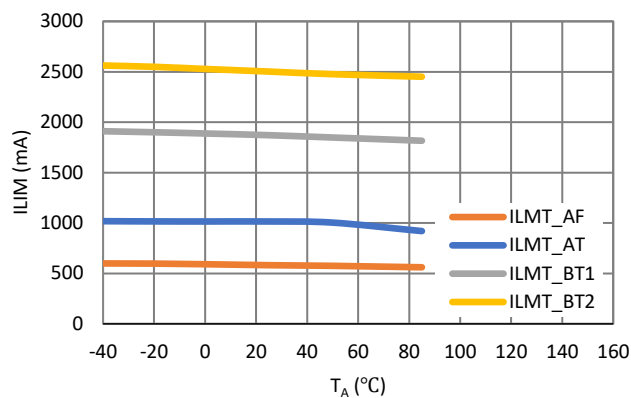
ILIM vs. Temperature
