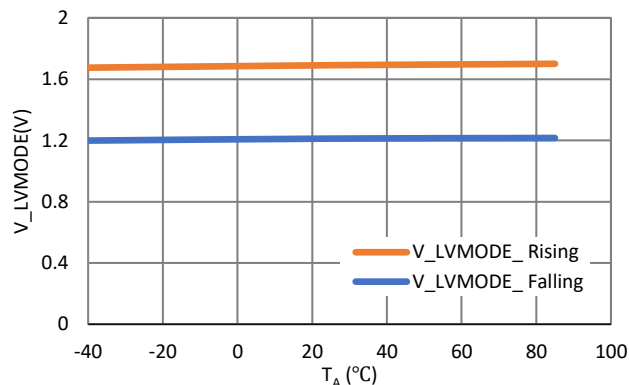
LVMODE Threshold vs. Temperature
