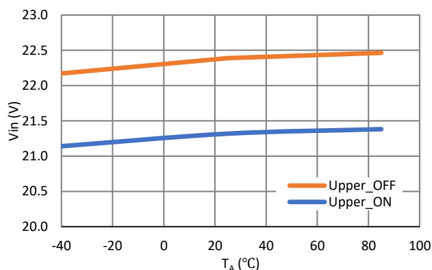
Class Upper Threshold vs. Temperature
