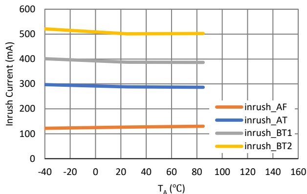
Inrush Current vs Temperature
