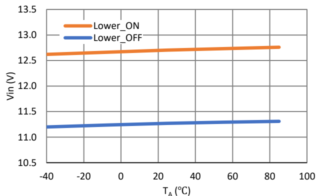
Class Lower Threshold vs. Temperature
