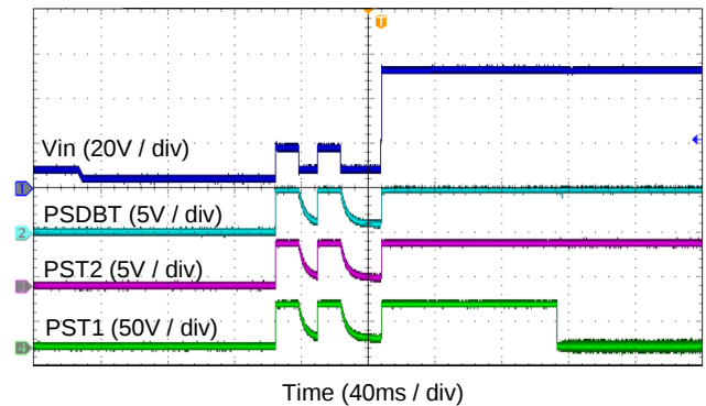
PoE. BT Detect at PSE12 Class4
