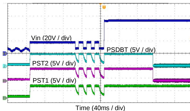
PoE. BT Detect at PSE34 Class5-6
