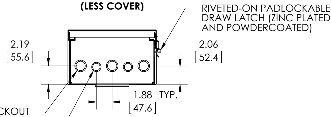
BOTTOM VIEW
