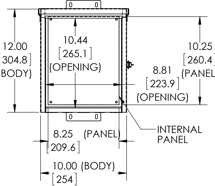
FRONT VIEW (LESS COVER)
