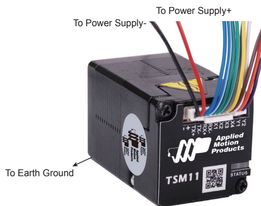
Standard Model
