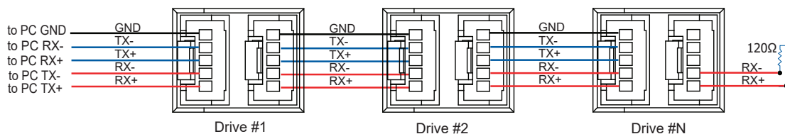
RS-422/485: 4-wire system diagram
