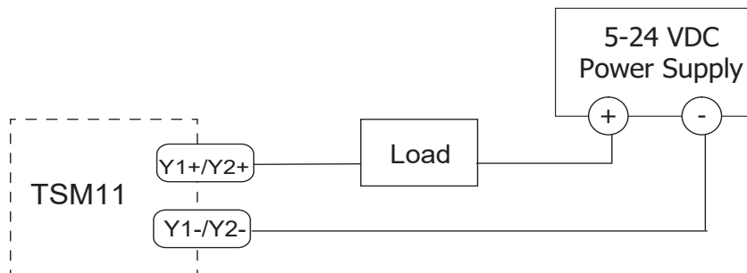
Connecting a Sinking Output
