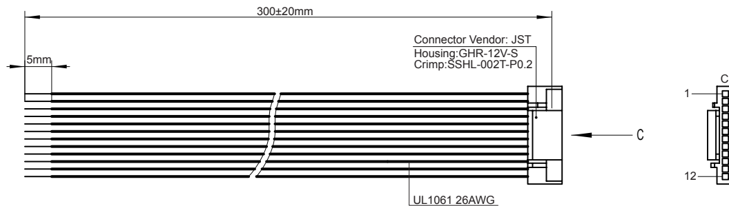
Mating Connector Diagram
