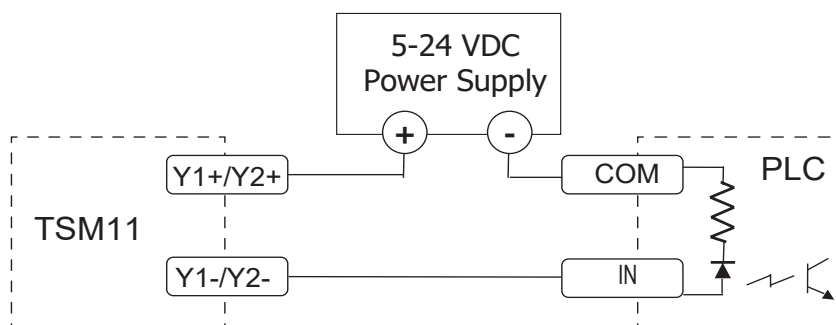
Connecting a Sourcing output with PLC's input
