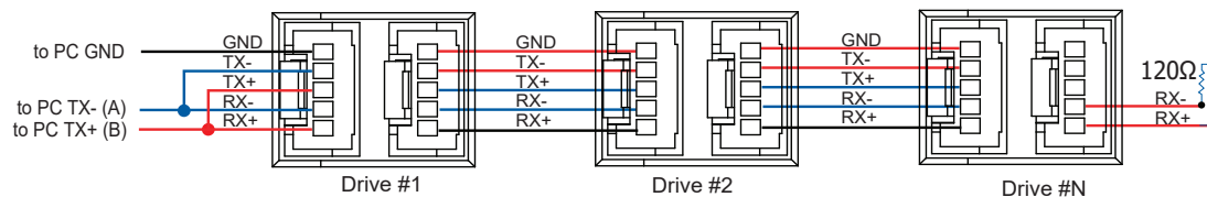
RS-422/485: 2-wire system diagram
