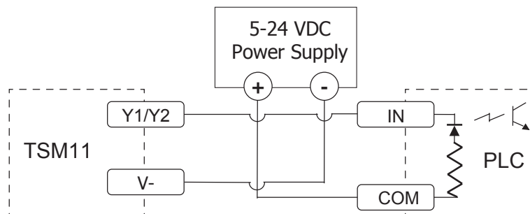
Connecting a sinking output with PLC's input
