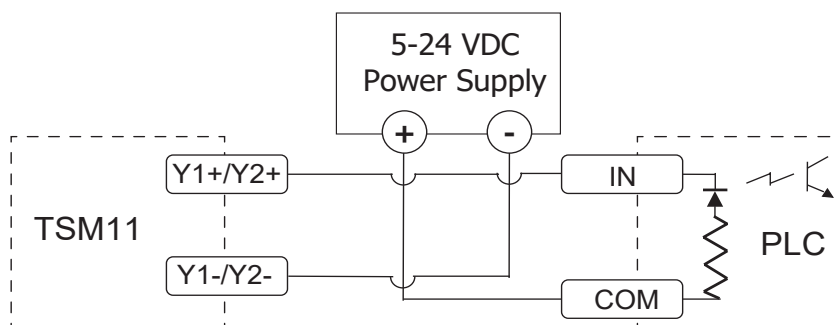
Connecting a sinking output with PLC's input
