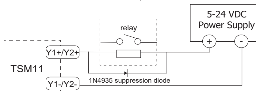
Driving a Relay
