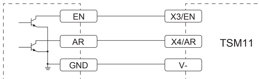
Connecting to Controller with Sinking Outputs
