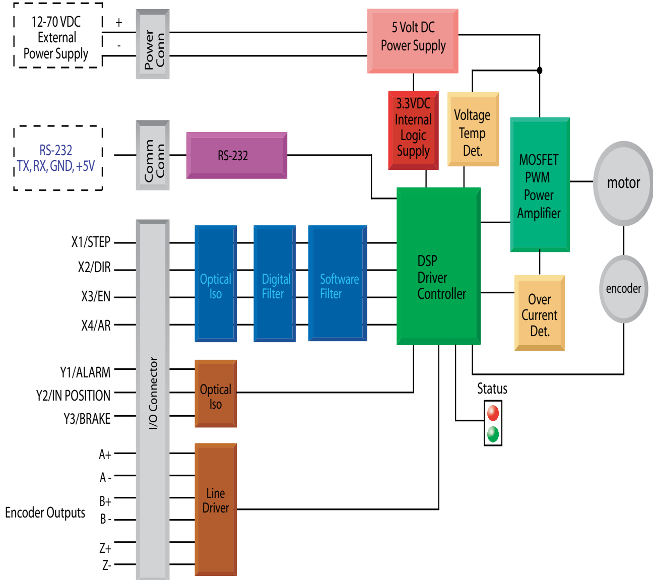
TSM23P Block Diagram
