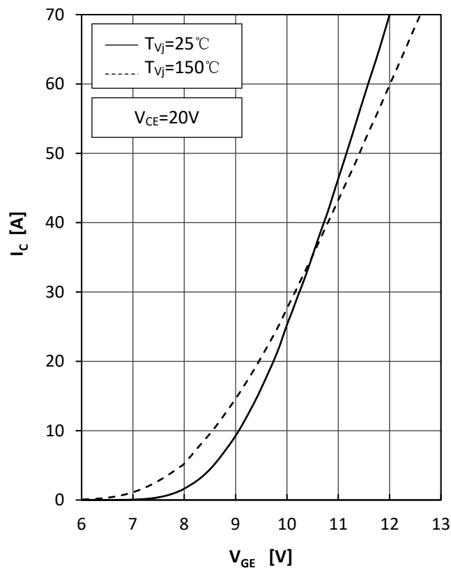
Fig2.IGBT Transfer Characteristics
