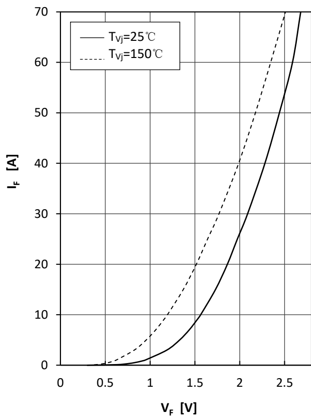
Fig7.Diode Foward Characteristics
